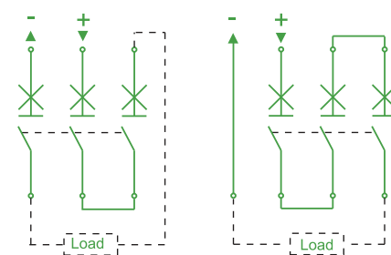
3 Poles
