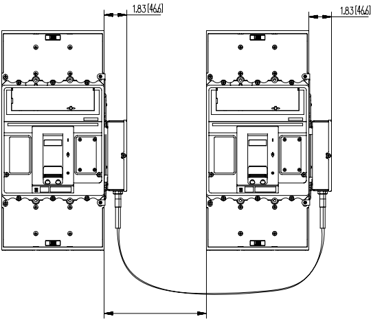
MIT26N Mechanical Interlock Unit: in [mm]
