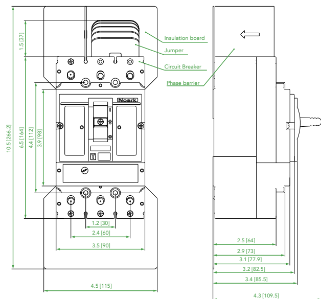
M1PVS Connection A Unit in [mm]
