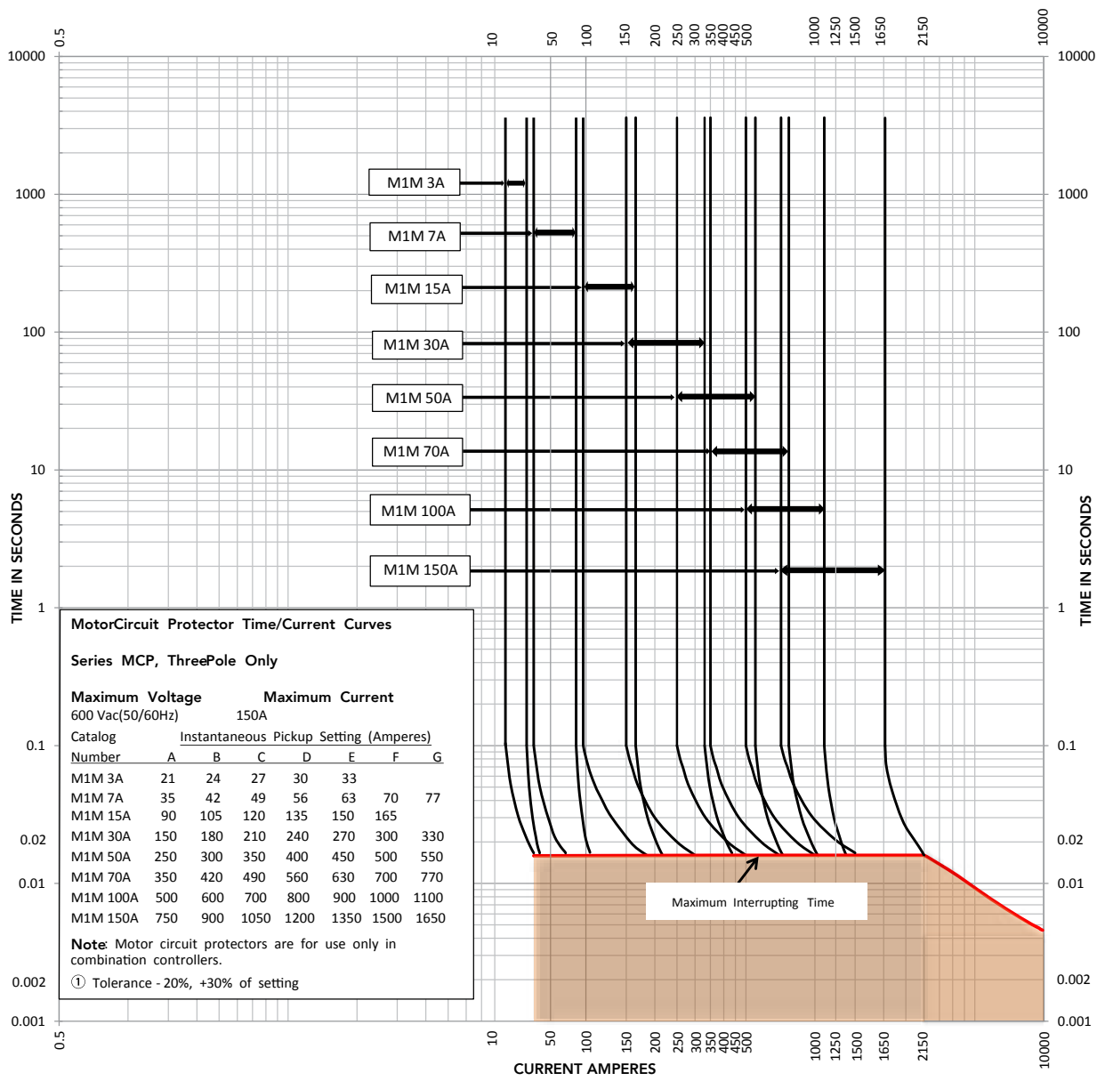
Motor Circuit Protector Time/Current Curves for M1M CURRENT AMPERES
