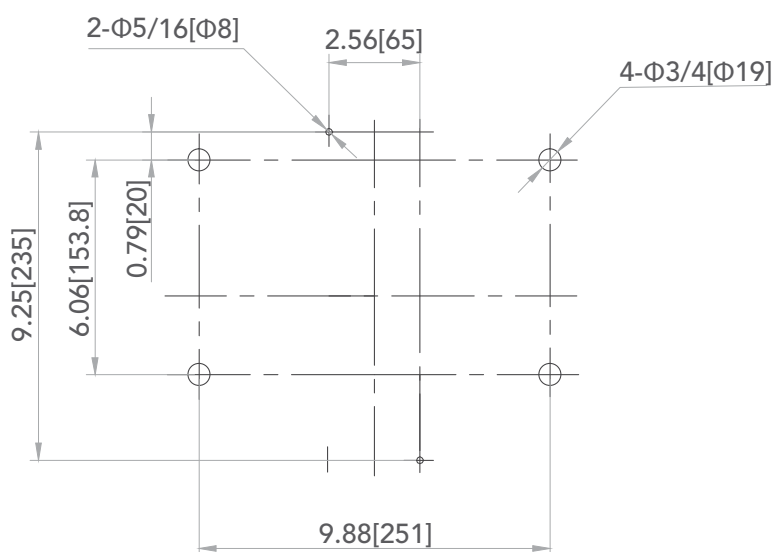
Drilling Plate for OM24
